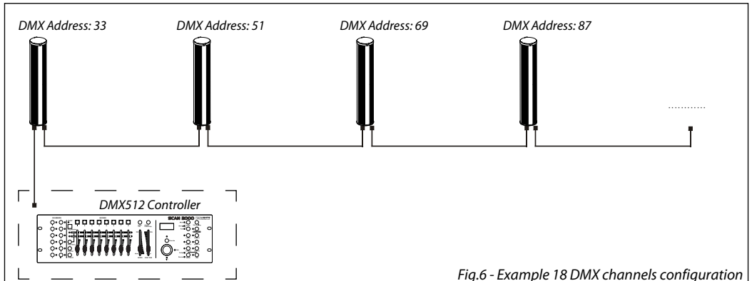
Fig.6 - Example 18 DMX channels configuration
