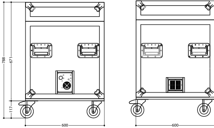
Technical drawing
